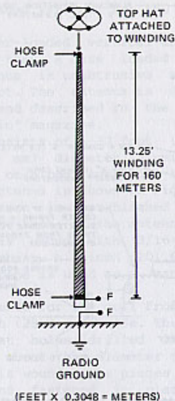
Fig. 14 Helix antenna for 160 meters is wound on tapered form. Small top hat is used to prevent high voltage corona discharge from top of the antenna.
