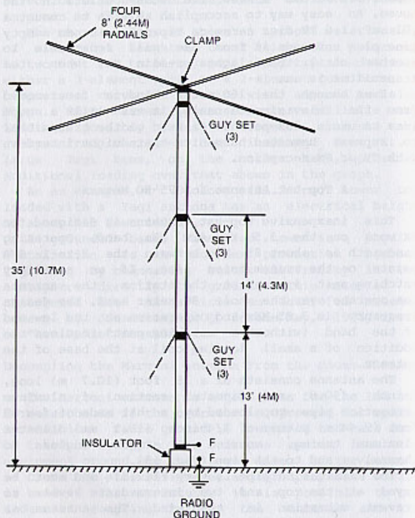
Fig. 19 Simple top hat antenna for 75-80 meters is only 35 feet high. Single section of aluminum irrigation pipe is used as radiator. Antenna is guyed at three points to prevent vibration in heavy wind.
