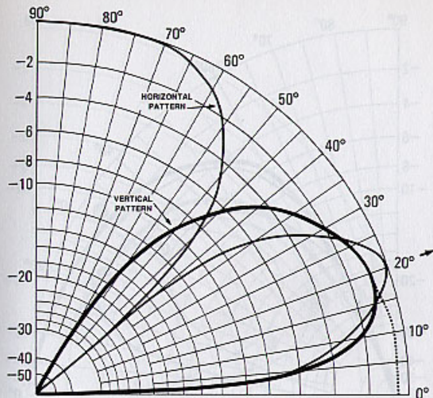
Fig. 6 A comparison of the vertical field patterns of horizontal and vertical antennas located above good ground. The horizontal antenna is 3/4-wavelength above ground while the base of vertical antenna is at ground level. Both antennas provide good radiation at a vertical angle of about 20 degrees but horizontal antenna must be 52 feet high to do the job on the 20 meter band.
