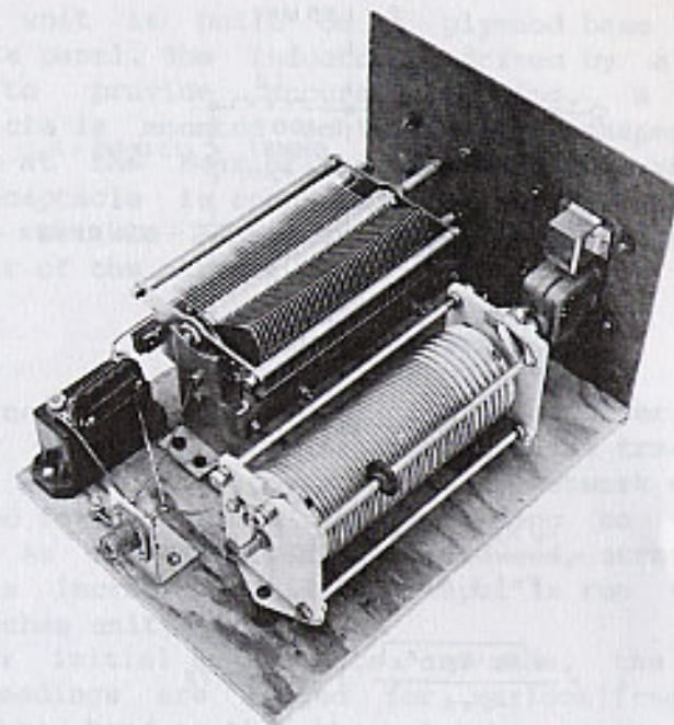
Fig. 8 L-network for 160 meters. Shunt capacitor is made up of large value air variable unit plus shunt-connected mica transmitting units. Rotary coil is large enough to take care of additional series loading inductance required by short Marconi antenna (see Fig. 9). Components are mounted on plywood base with fiberboard panel. Counter dial is coupled to rotary inductor.
