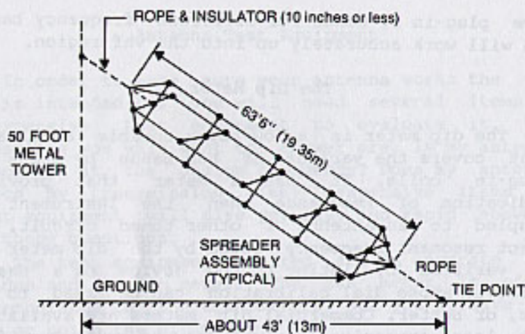
Fig. 4 Broadband sloper antenna for 80 meters. Spreaders are made of 3/8 inch (9.2cm) fiberglass rods. All wires are connected by jumpers at each spreader. SWR is less than 1.4-to-1 over 3.5 to 4.0 MHz.
