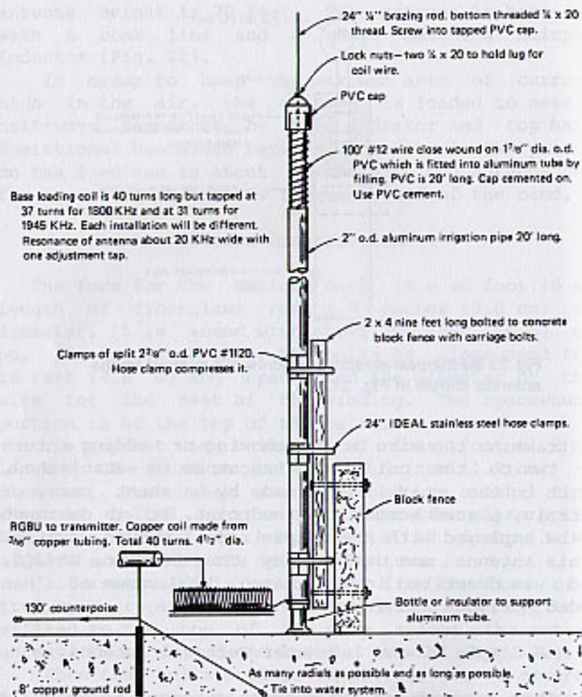
Fig. 23 Inexpensive vertical antenna for 80 and 160 meter operation. Top loading coil resonates antenna to 80 meters and bottom coil adds extra loading for 160 meters. Antenna is made of 20 foot length of aluminum irrigation pipe.
