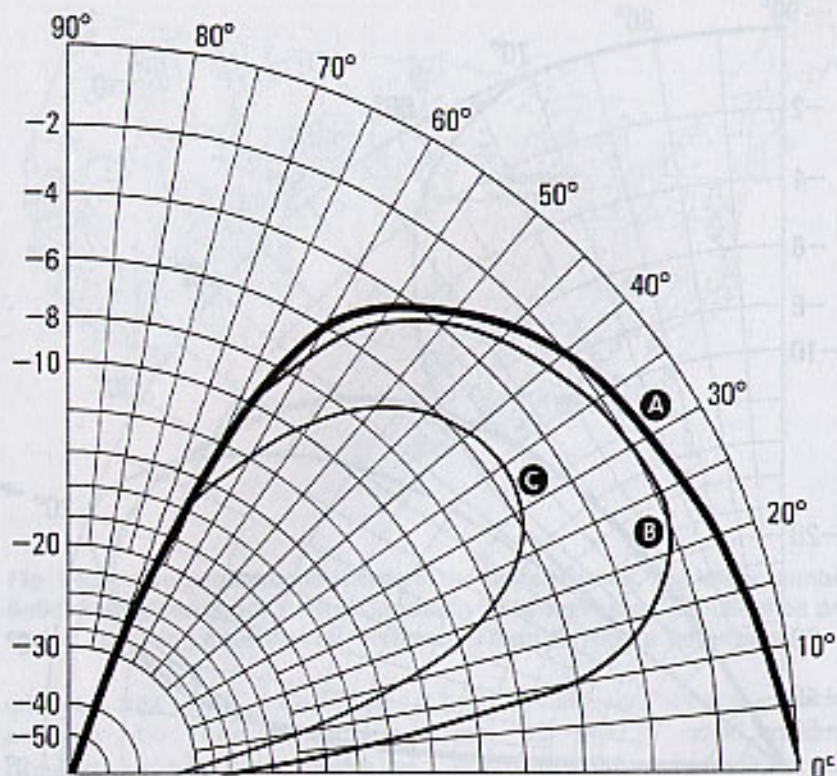
Fig. 7 Vertical radiation pattern of a vertical dipole whose base is at ground level. Over perfect ground, low angle radiation is maximum at the horizon (A). Over average ground (B), typical of the United States, some extremely low angle radiation is lost. Poor ground conductivity (C) reduces radiation at all vertical angles.
