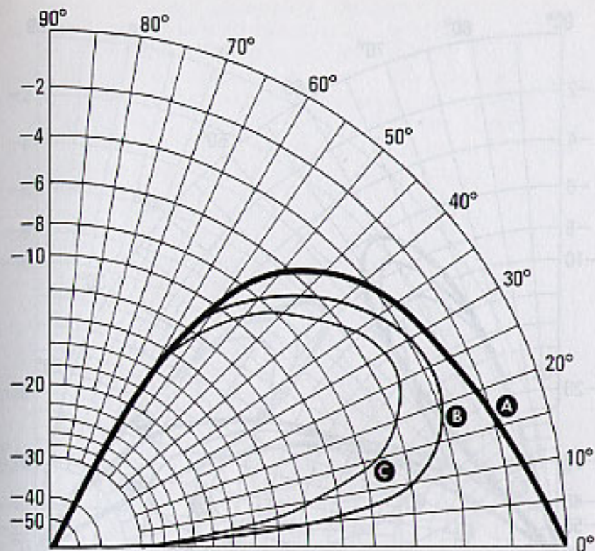
Fig. 8 Vertical radiation pattern of a ground plane antenna with the base at ground level resembles vertical dipole pattern, with ground absorption losses showing below about 15 degrees. A = perfect ground, B = average ground, C = poor ground.
