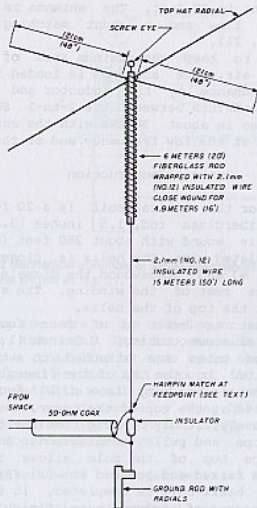
Fig. 21 Tree- or tower-mounted vertical antenna for 160 meters. Top hat and helix structure are supported by screw eye at top and connected to feedpoint with vertical wire.
