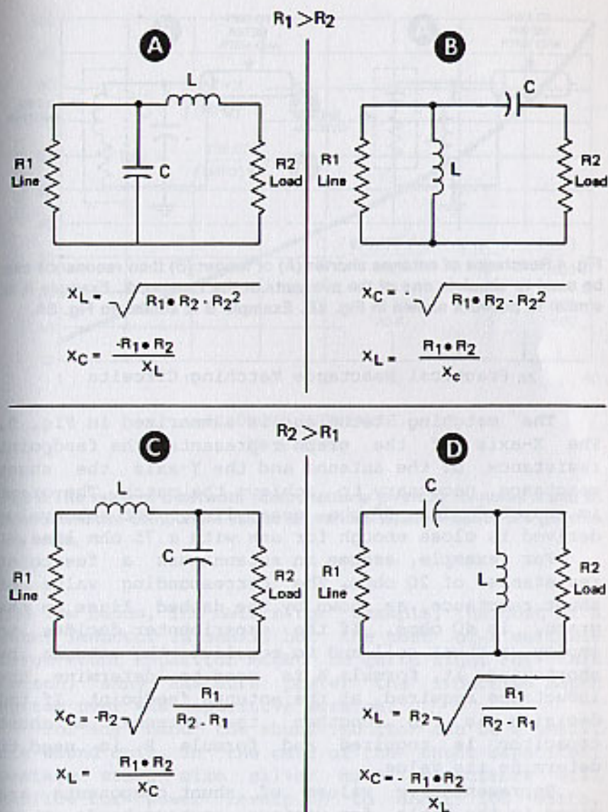
Fig. 3 Basic L-networks used to match antenna to feedline. Networks A and B are used when coax line impedance is greater than feedpoint impedance. Networks C and D are used when feedpoint resistance is greater than coax impedance.
